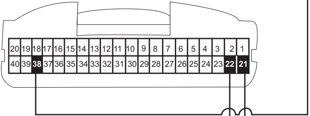
Front view of the BCM connector located on the driver kick panel or above the acceleration pedal.
